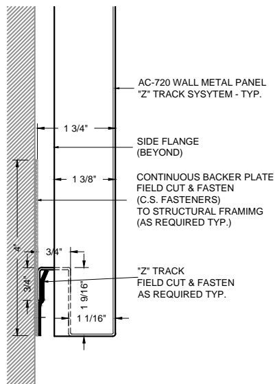
5 PERIMETER DETAIL (BASE) AC-720-FB1
