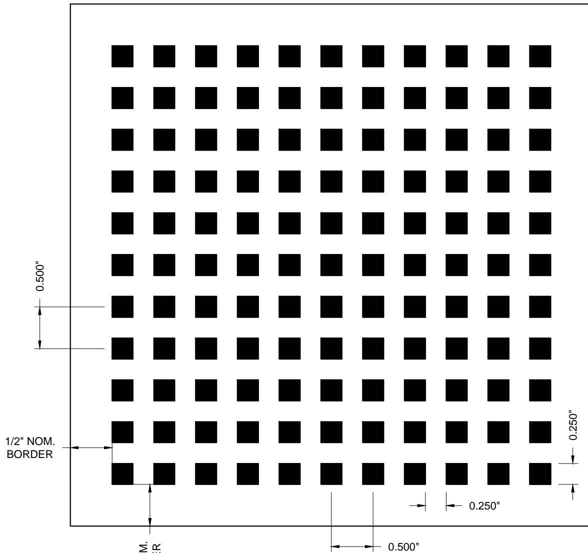
PERFORATION S250-25-1 1/4" SQUARE @ 1/2" STRAIGHT CENTERS (25% OPEN)
