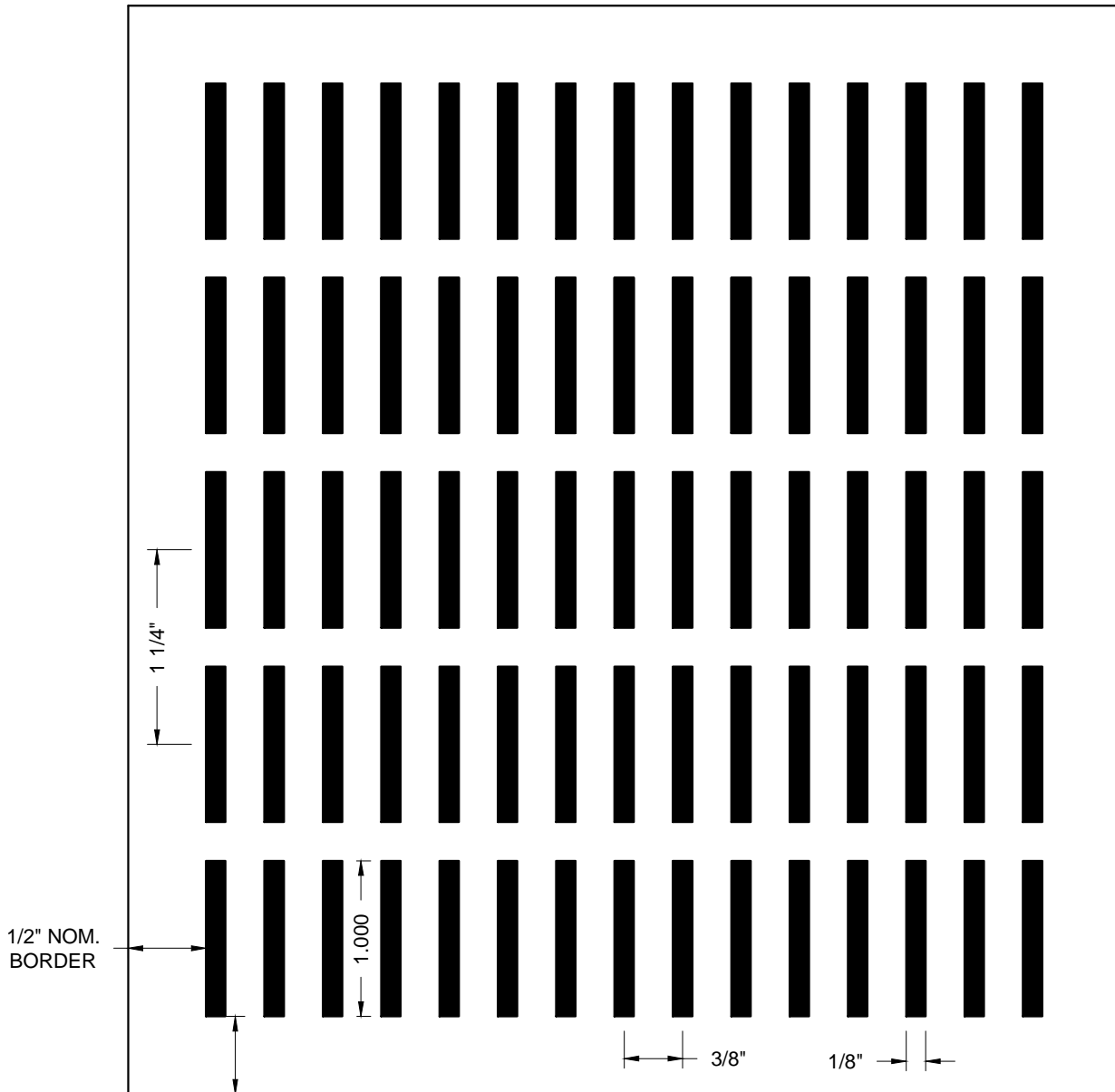
PERFORATION, RT125x100-26-1 1/8" x 1" RECTANGULAR SLOT @ 3/8" x 1-1/4" STRAIGHT CENTERS (26% OPEN)
