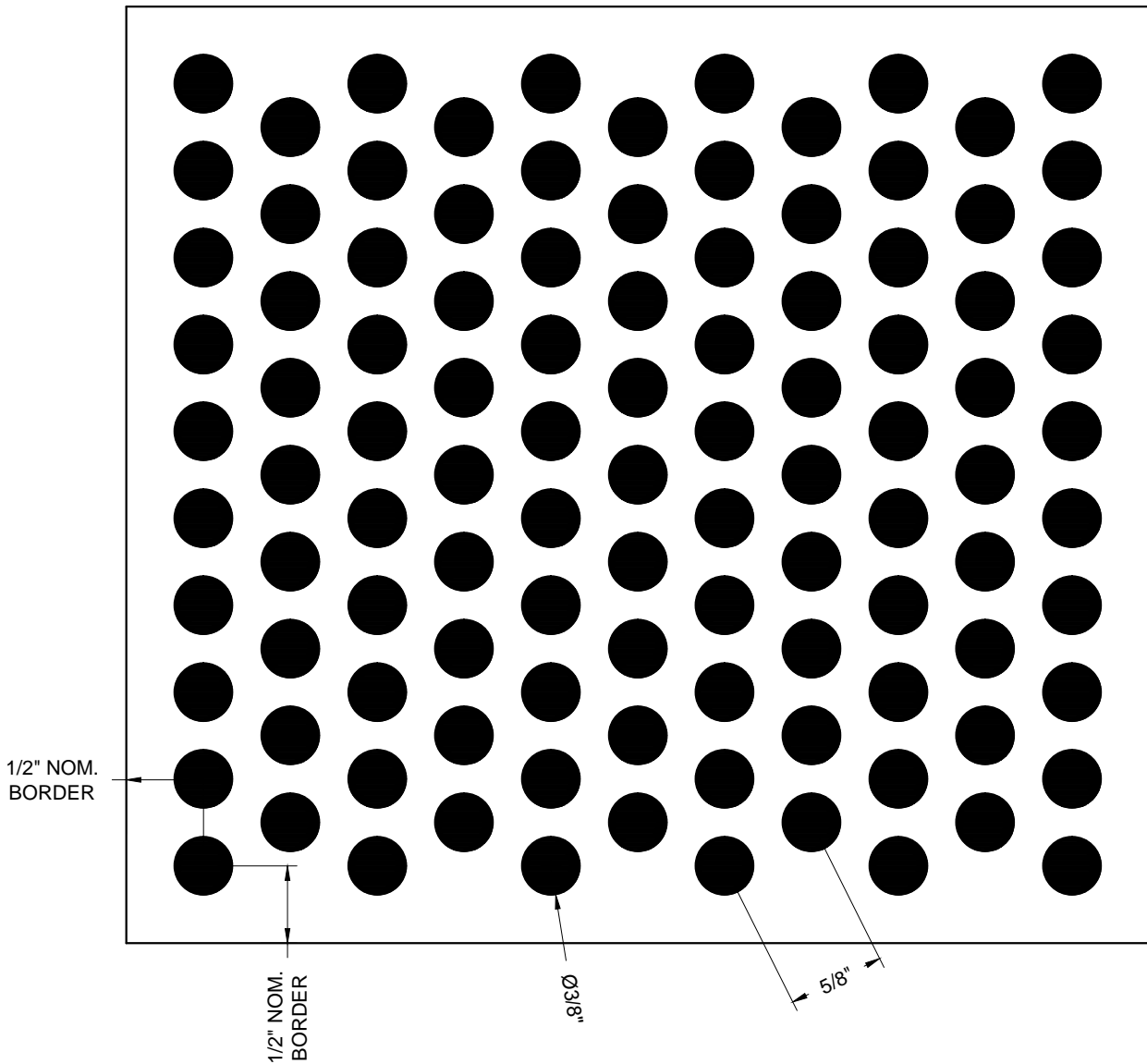
PERFORATION R375-40-5 3/8" DIA. HOLES @ 5/8" CUSTOM STAGGERED CENTERS (40% OPEN)
