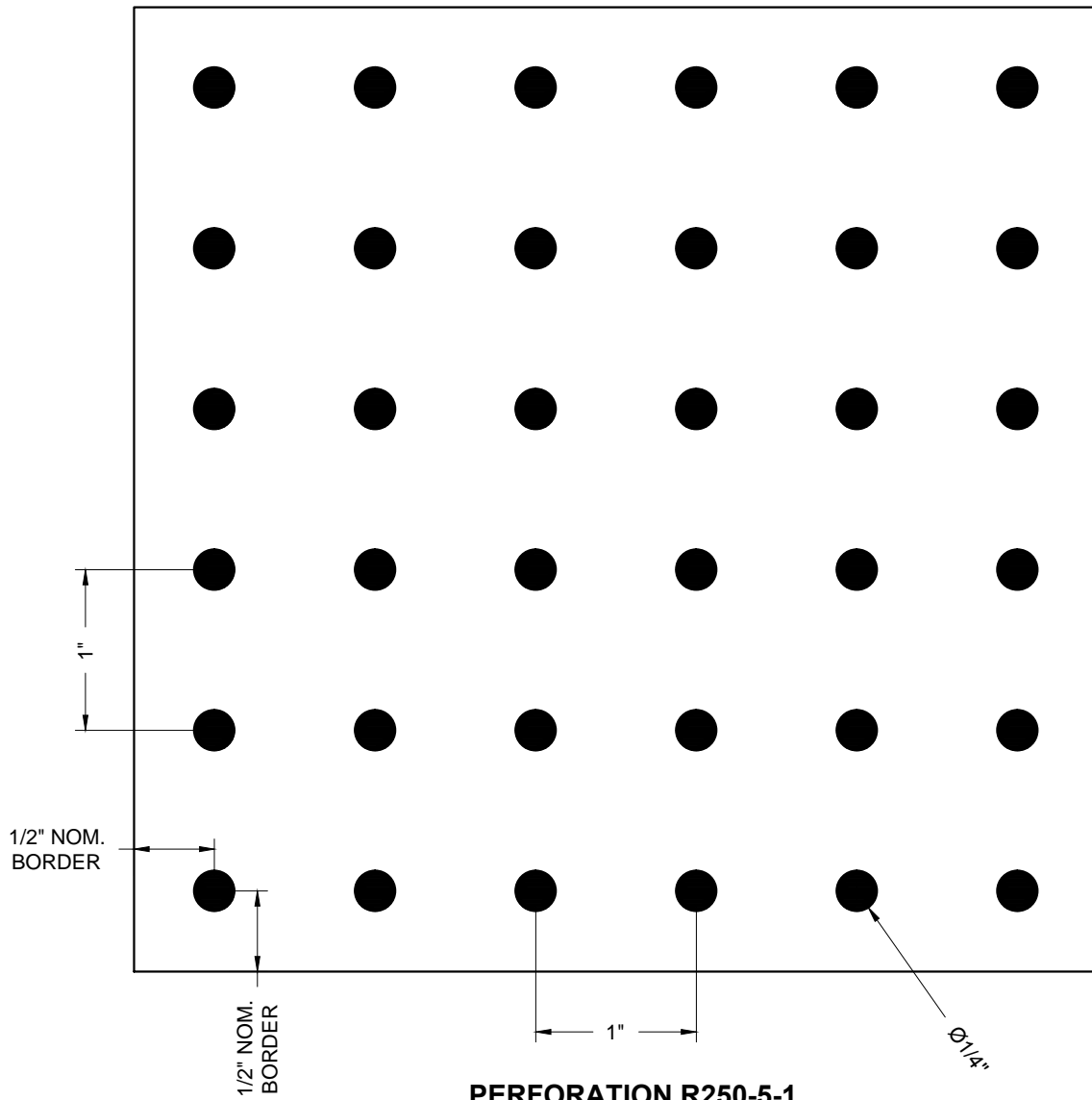
PERFORATION R250-5-1 1/4" DIA. HOLES @ 1.00" STRAIGHT CENTERS (5% OPEN)
