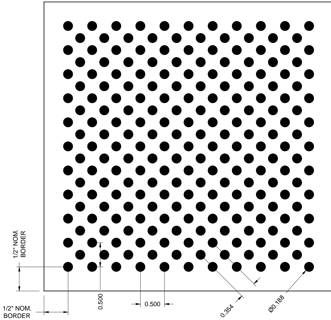
PERFORATION R188-22-3 .188 DIA. HOLES @ .354 STAGGERED CENTERS (22% OPEN)
