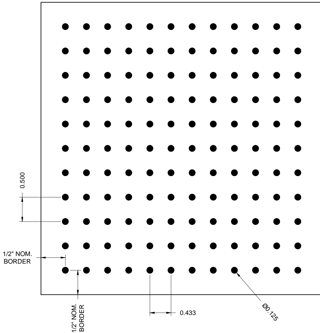
PERFORATION R125-06-1 .125 DIA. HOLES @ .433 x .500 STRAIGHT CENTERS (6% OPEN)
