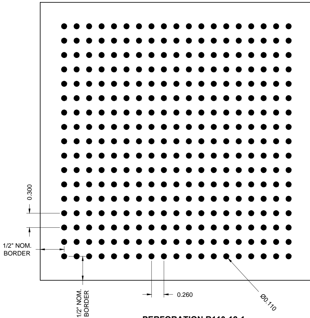
PERFORATION R110-12-1 .110 DIA. HOLES @ .260 x .300 STRAIGHT CENTERS (12% OPEN)
