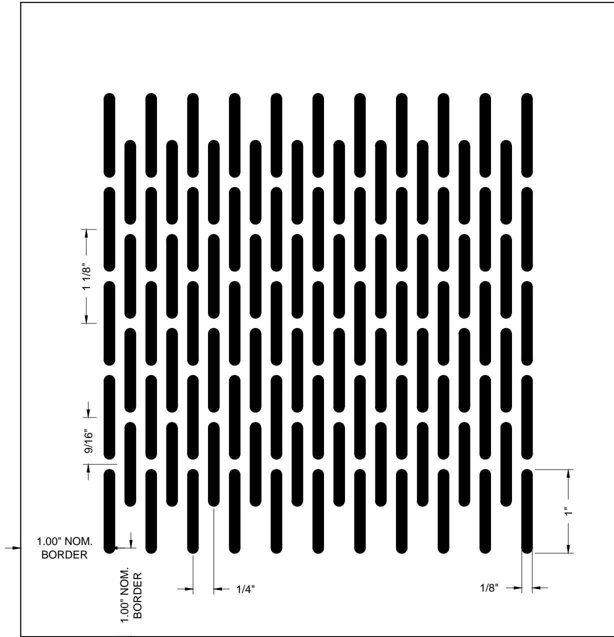
PERFORATION OB,125x1000-43-2 1/8" x 1.00 OBOURD SLOT @ 1/4" x 9/16" STAGGERED CENTERS (43% OPEN)
